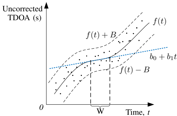
Fig. 5: f(t) represents the clock skew difference between the two hydrophone clocks. The two dotted curves represent the maximum and minimum TDOA measurements given the skew. b_0 + b_1 t represents the local clock skew function obtained by solving the MILP formulation over the window of size W .
